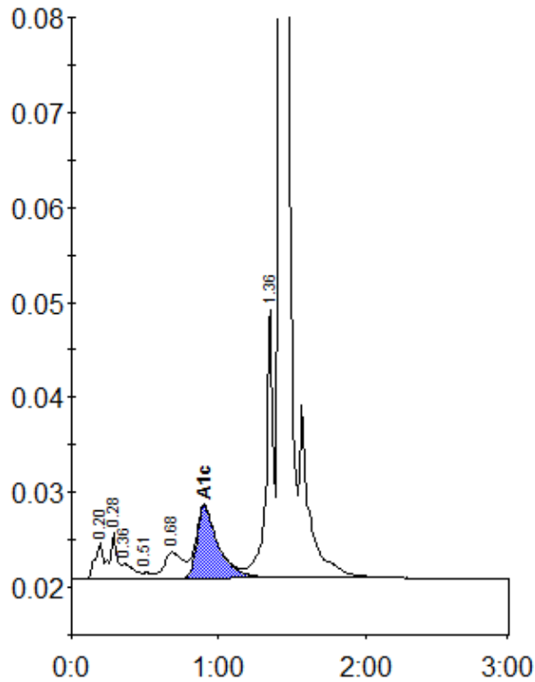
Peak table - ID: 10486541
